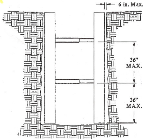
TRENCH CROSS SECTION
