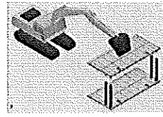
LOWER SECOND SIDEWALL ON TO SPREADERS AND PIN
